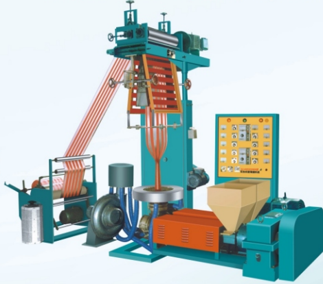
SJ-45X2 双色彩条吹膜机 SJ-45X2 Double-colour Striped Film Blowing Machine
